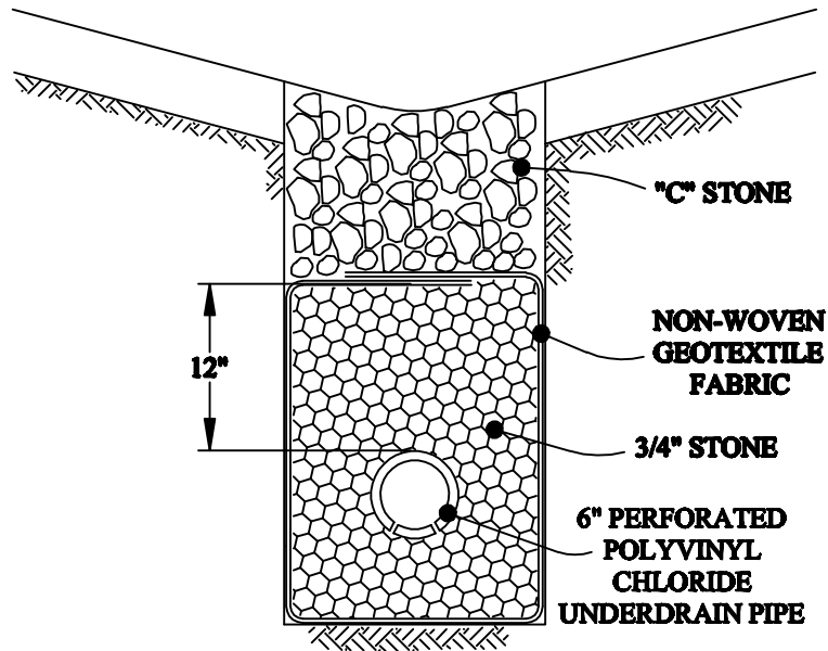
Ditch Section
