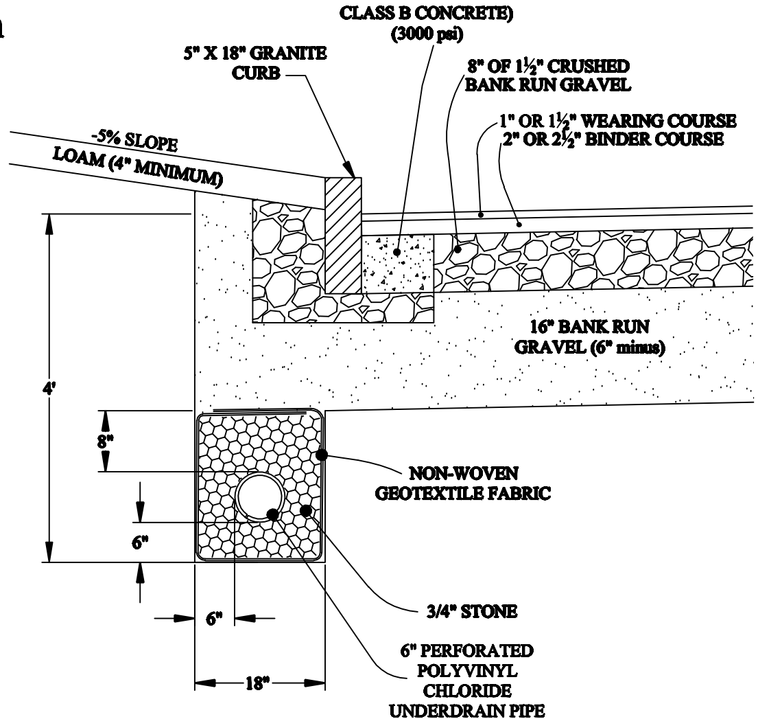
Road Section (WITH CURB)
