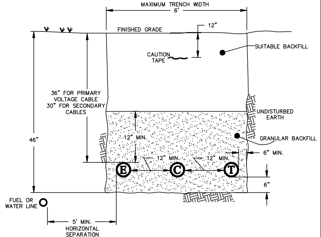
TYPICAL TRENCH CROSS-SECTION WITH SIDE-BY-SIDE CONDUIT CONFIGURATION (N.T.S.)
