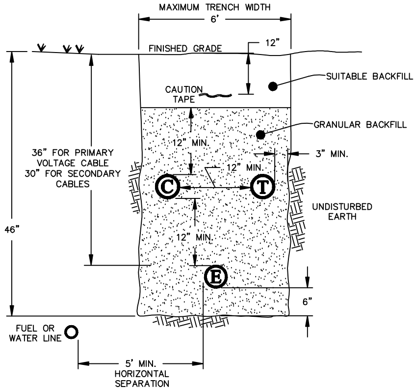
TYPICAL TRENCH CROSS-SECTION WITH STACKED CONDUIT CONFIGURATION (N.T.S.)
