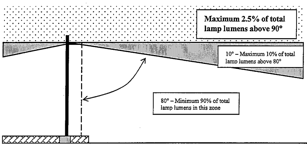
Cut-off fixture as defined by IESNA.
